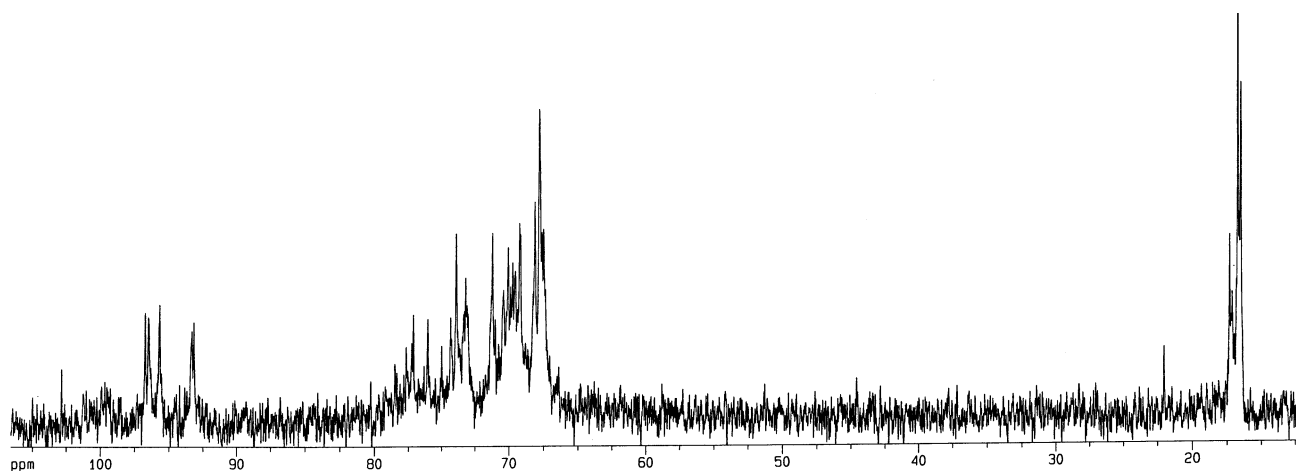
Fig. 7. ^{13}\text{C} NMR spectrum of native fucoidan from C. filum A-2.
