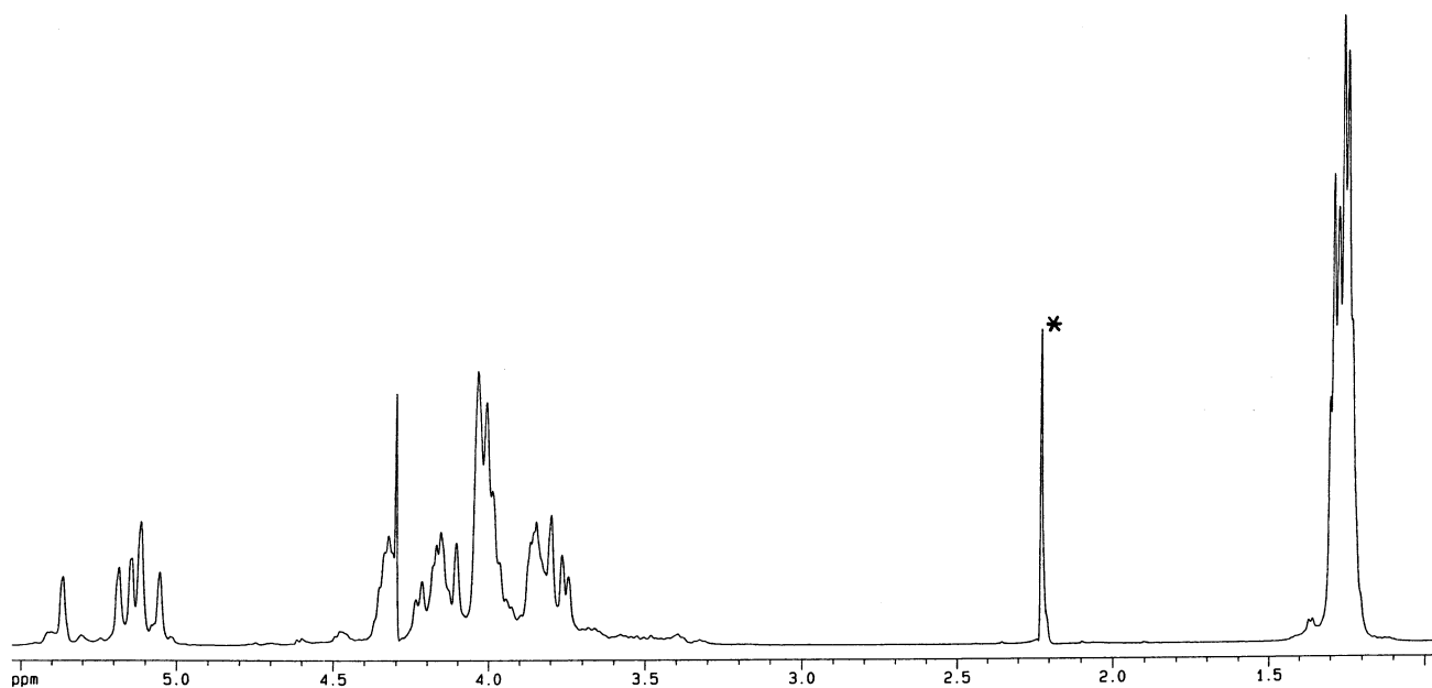
Fig. 4. ^1\text{H} NMR spectrum of desulfated, deacetylated fucoidan DD-2. * Acetone signal (see text and Table 3 for assignments).
