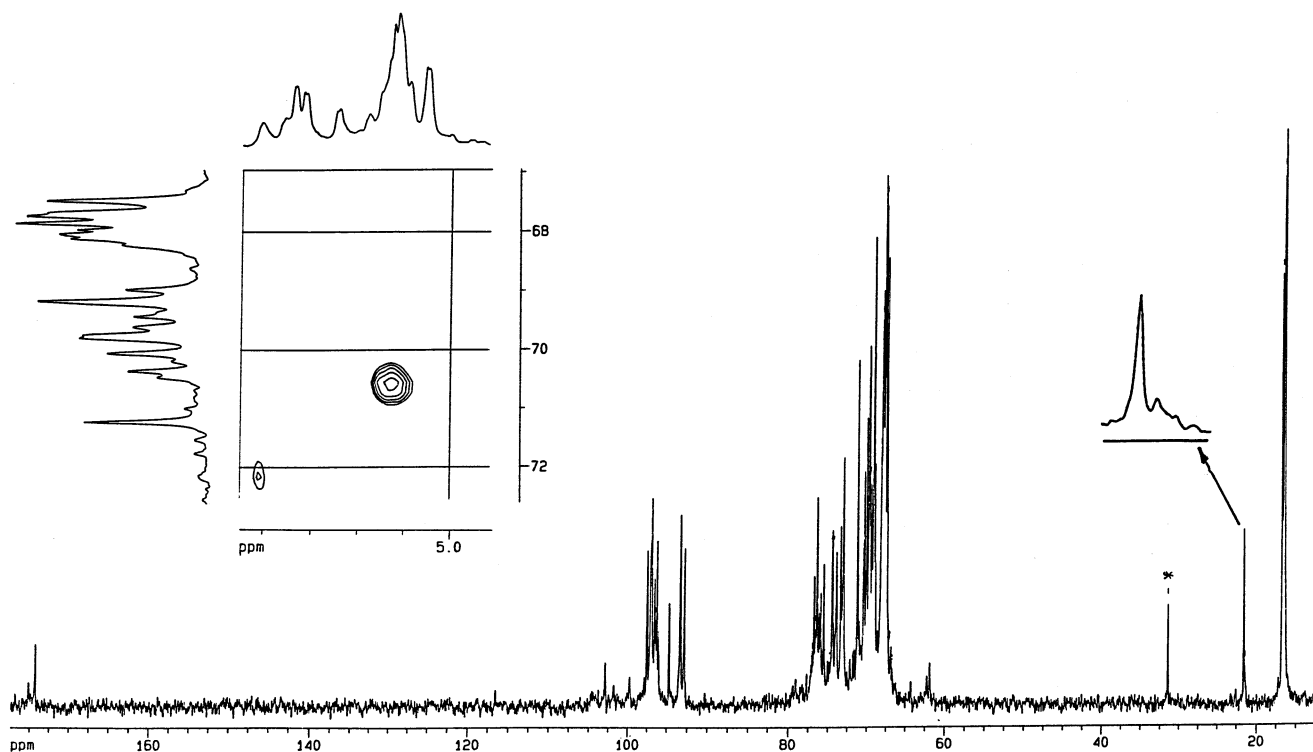
Fig. 2. ^{13}\text{C} NMR spectrum of desulfated fucoidan D-2. * Acetone signal. A fragment of HMQC spectrum is presented in an inset (left) to prove the presence of O -acetate. The acetate \text{CH}_3 area is expanded (right inset) (see text for details).
