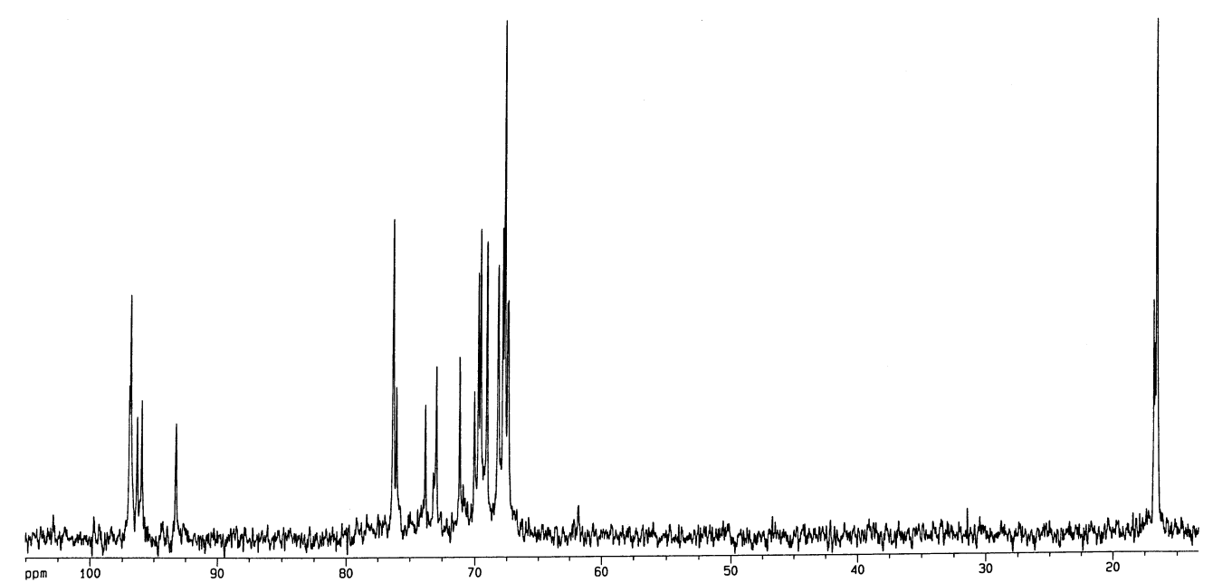
Fig. 3. 13 C NMR spectrum of desulfated, deacetylated fucoidan DD-2 (see text and Table 2 for assignments).
