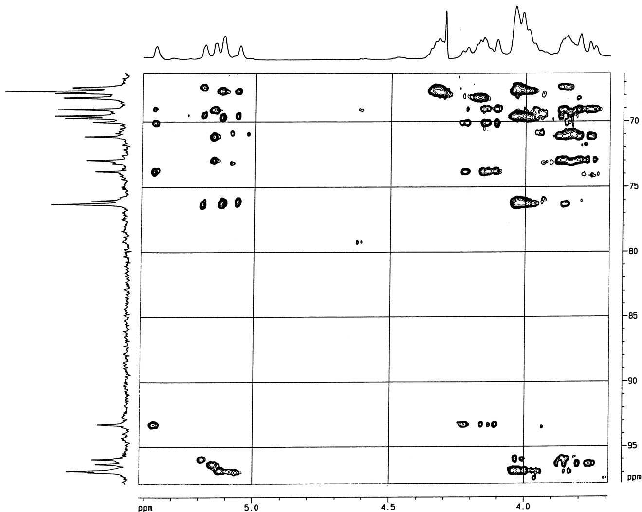
Fig. 5. HMQC-TOCSY NMR spectrum of desulfated, deacetylated fucoidan DD-2 (see text for details).
