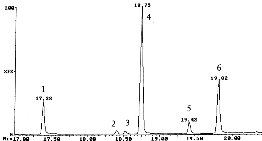
Fig. 1. GLC-MS of partially methylated alditol acetates derived from desulfated fucoidan D-2 (TIC chromatogram). 1, 1,5-Di- O -acetyl-2,3,4-tri- O -methylfucitol; 2, 1,4,5-tri- O -acetyl-2,3-di- O -methylxylitol; 3, 1,4,5-tri- O -acetyl-2,3-di- O -methylfucitol; 4, 1,3,5-tri- O -acetyl-2,4-di- O -methylfucitol; 5, 1,3,4,5-tetra- O -acetyl-2- O -methylfucitol; 6, 1,2,3,5-tetra- O -acetyl-4- O -methylfucitol.
