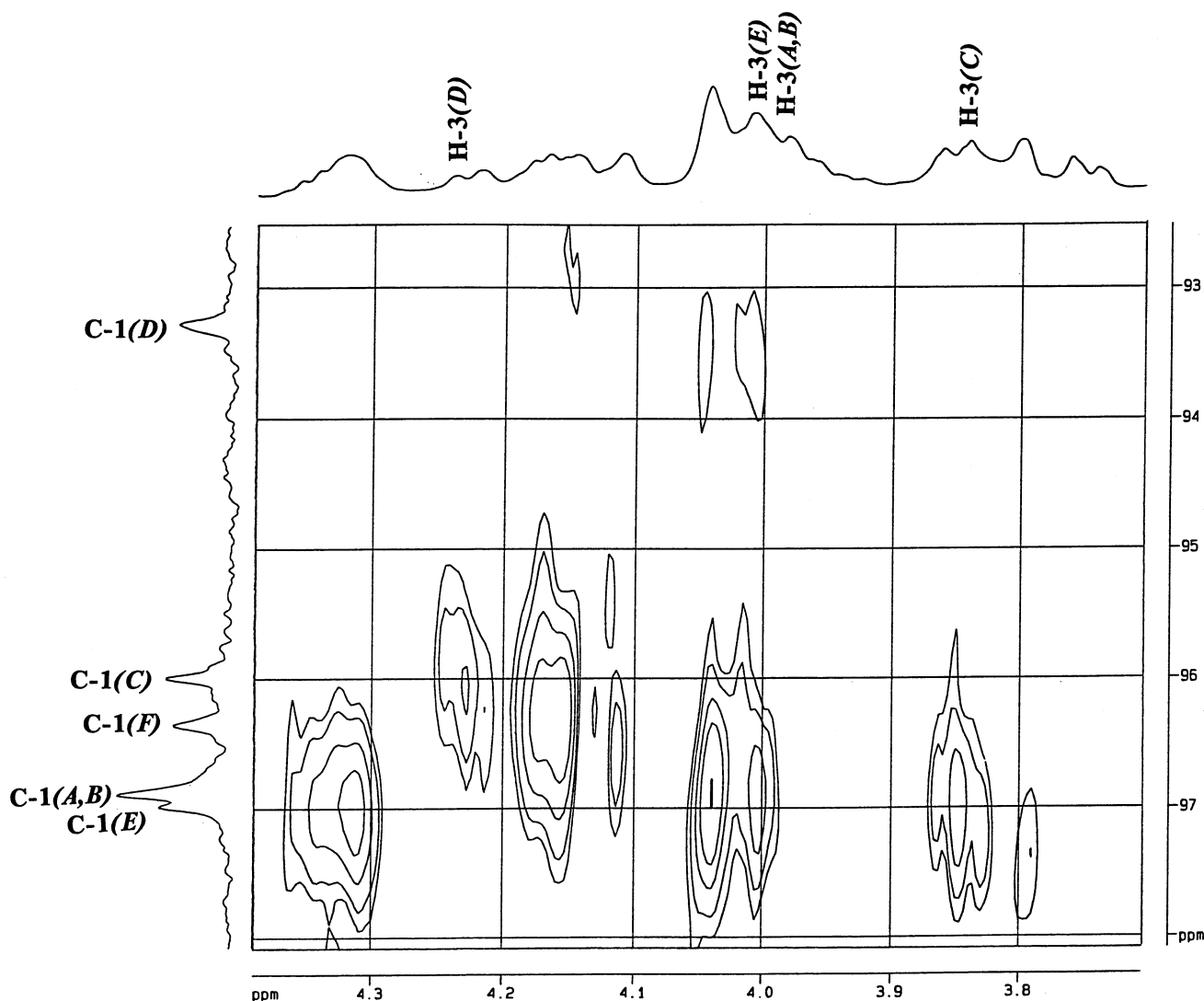
Fig. 6. 2D HMBC NMR spectrum (in part) of desulfated, deacetylated fucoidan DD-2 (see text for details).
